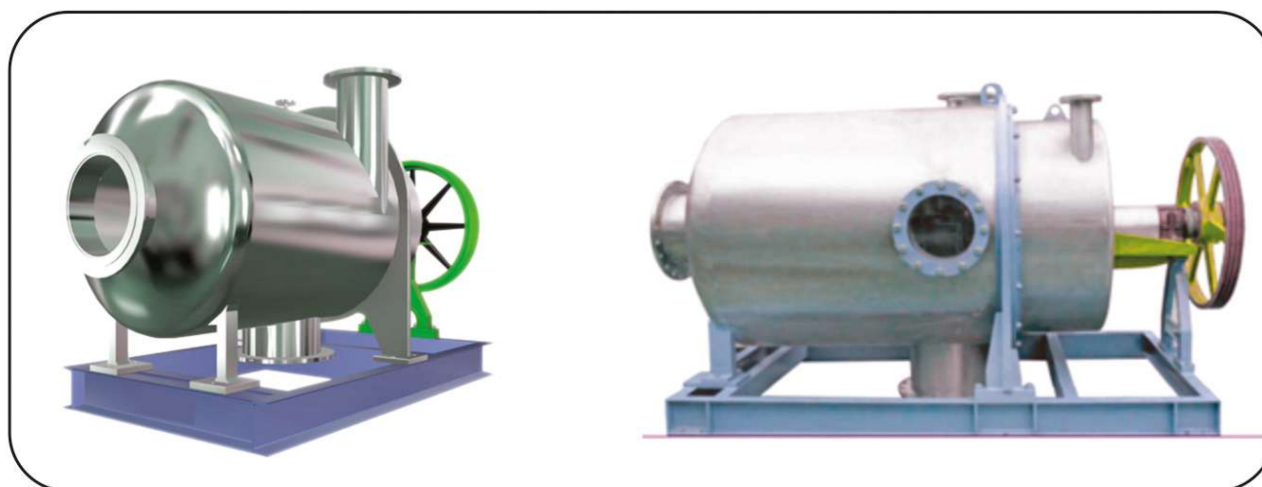
FIBER SAVER
